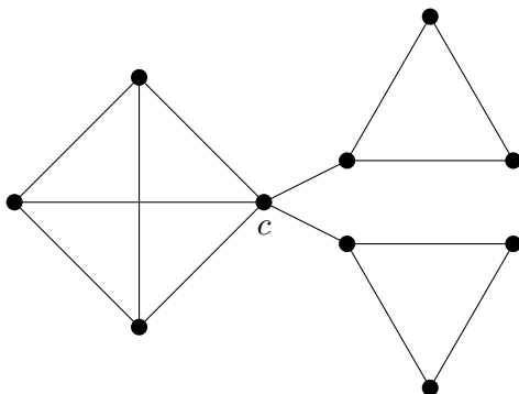
Figure 2: The Turán connected graph \text{TC}_{10,3} .
