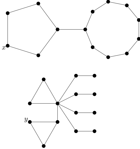
Figure 4: The remaining case in the proof of Theorem 3.1 (for n = 14 ).
