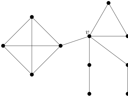
Figure 3: An almost Turán connected graph.
