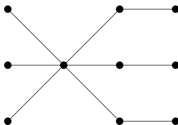
Figure 5: The Turán connected graph \text{TC}_{10,6} , which is a tree.
