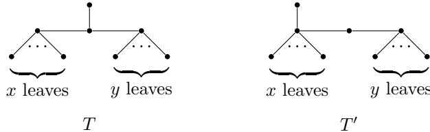
FIGURE 1. The trees T and T'
