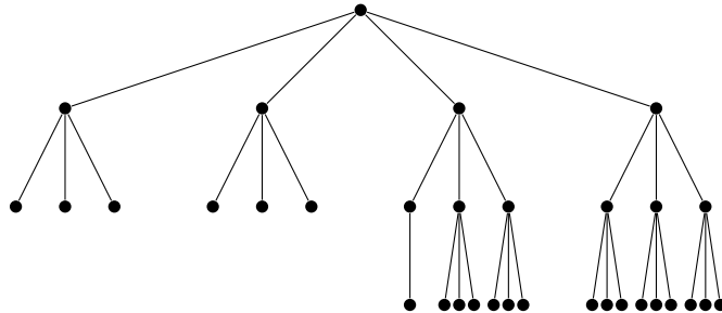
FIGURE 6. A complete 4-ary tree
