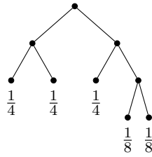
FIGURE 2.1. The canonical tree associated with the partition/composition 1 = 3 \cdot 2^{-2} + 2 \cdot 2^{-3} of 1 into powers of 2. This partition has weight \frac{1}{12} and corresponds to 10 distinct compositions.
